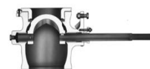
V200 VALVE
