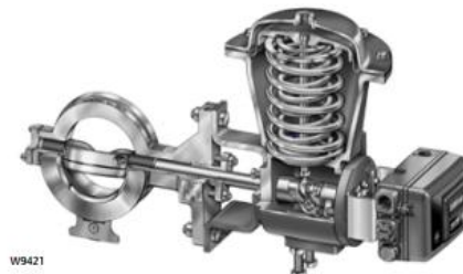
Control-Disk VALVE
