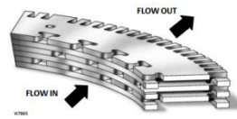
Figure 2. Typical WhisperFlo Trim Cut Section View for Fisher HP Valve
