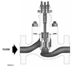
Figure 1. Fisher HPD Valve Assembly (NPS 2 to 6)
