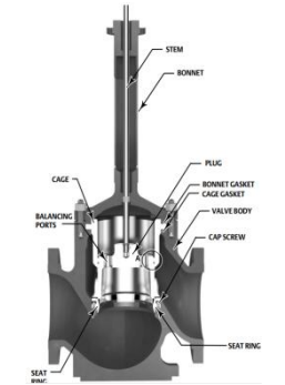
Figure 1. Typical Fisher ED/EWD Valve
