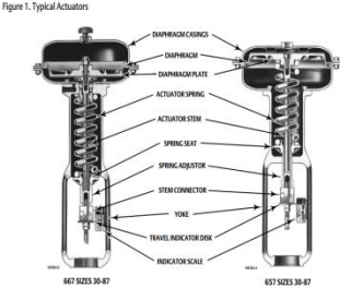
Figure 1. Typical Actuators
